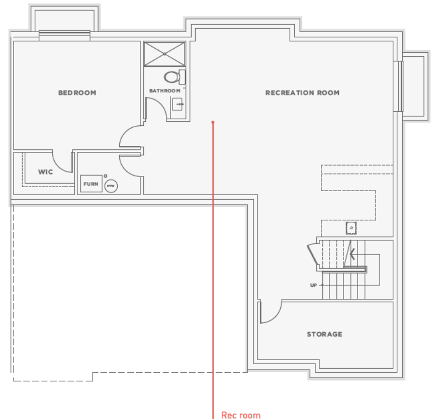
LOWER FLOOR 1,339 SQFT
