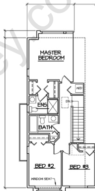
THIRD FLOOR PLAN 104 S.F.
