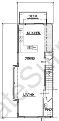
SECOND FLOOR PLAN 106 S.F.
