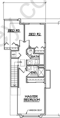
THIRD FLOOR PLAN
