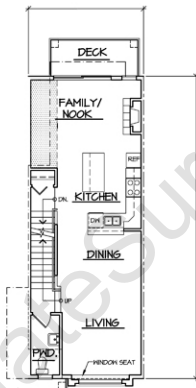
SECOND FLOOR PLAN 674 S.F.
