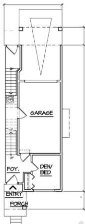
GROUND FLOOR PLAN 294 S.F.
