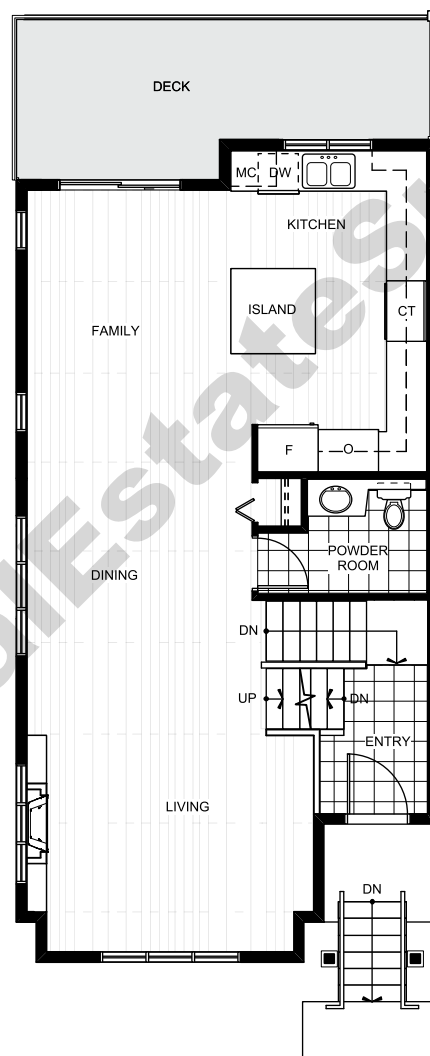
MAIN FLOOR 792 SQ. FT.
