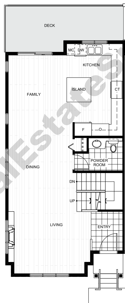
MAIN FLOOR 808 SQ. FT.
