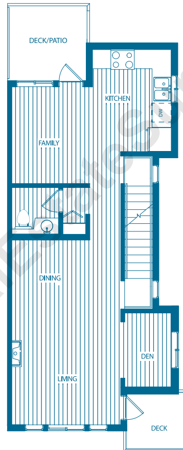
MAIN FLOOR
