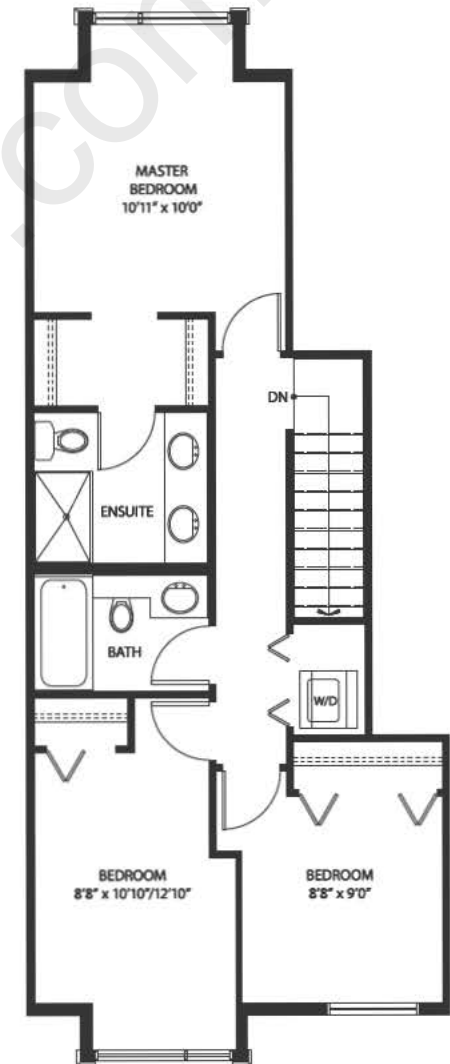
UPPER LEVEL 647 Sq Ft
