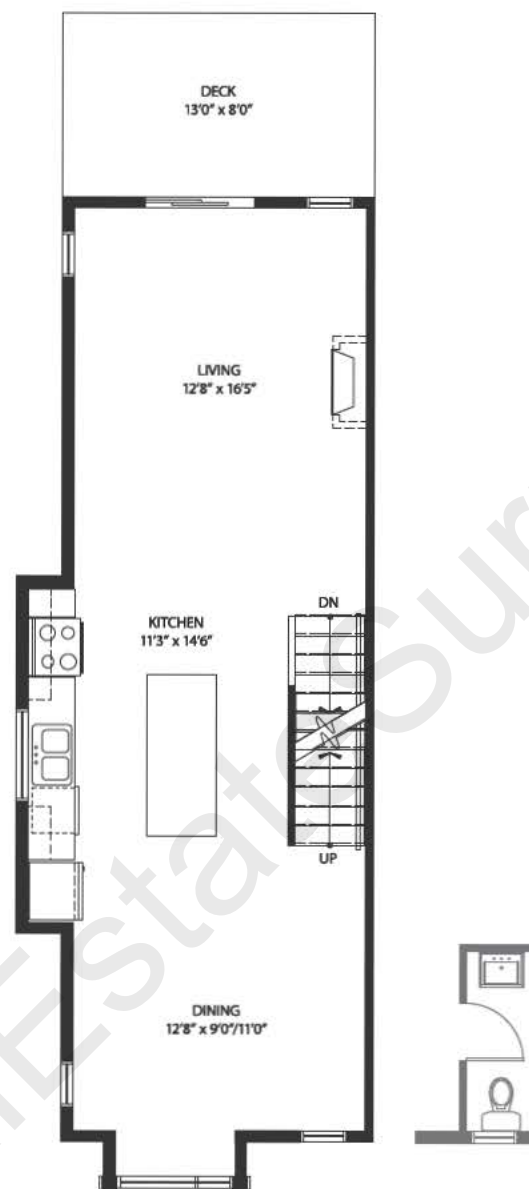
MAIN LEVEL 596 Sq Ft
