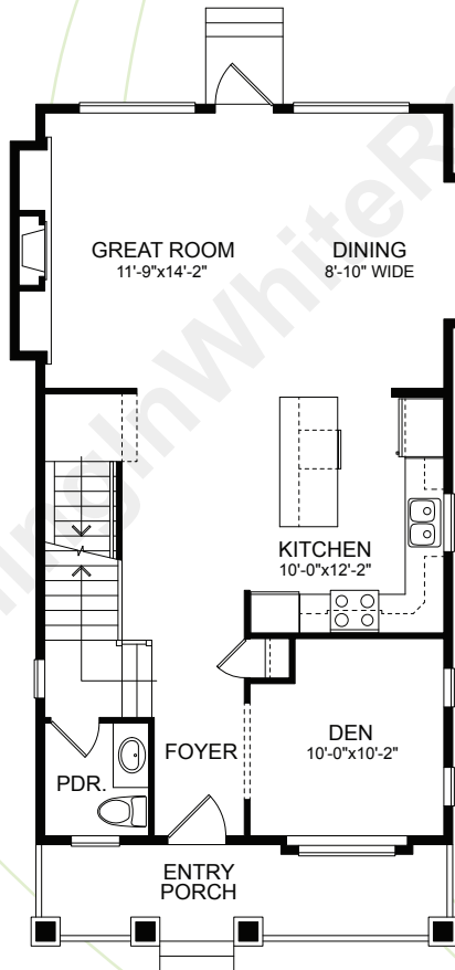
MAIN FLOOR PLAN 854 sq.ft.
