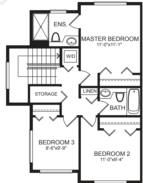
UPPER FLOOR PLAN 709 sq.ft.
