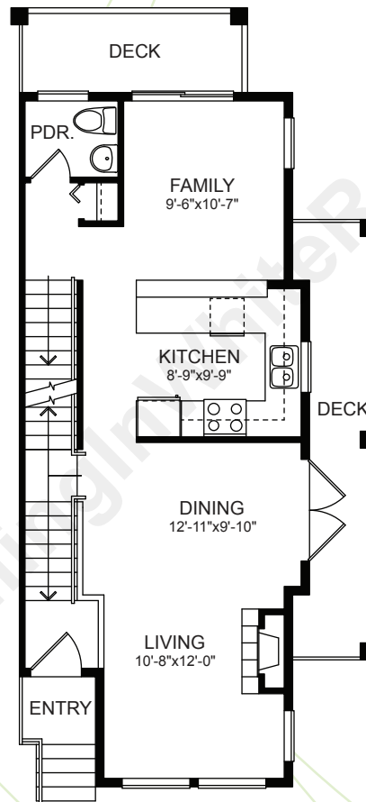
MAIN FLOOR PLAN 652 sq.ft.
