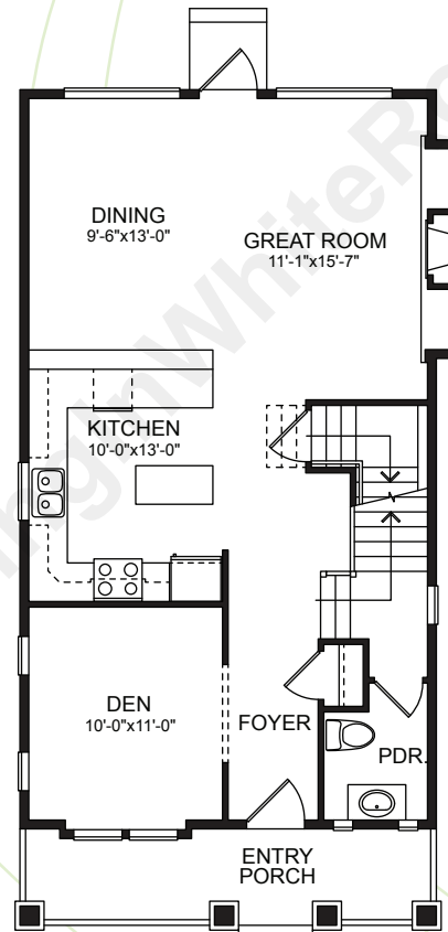
MAIN FLOOR PLAN 846 sq.ft.
