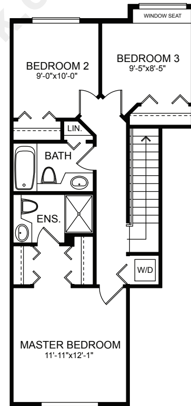
UPPER FLOOR PLAN 663 sq.ft.
