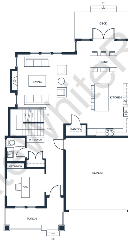
MAIN FLOOR 1,157 SQ FT
