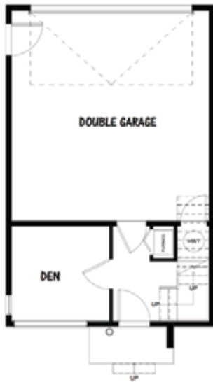
LEVEL 1
