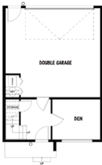
LEVEL 1
