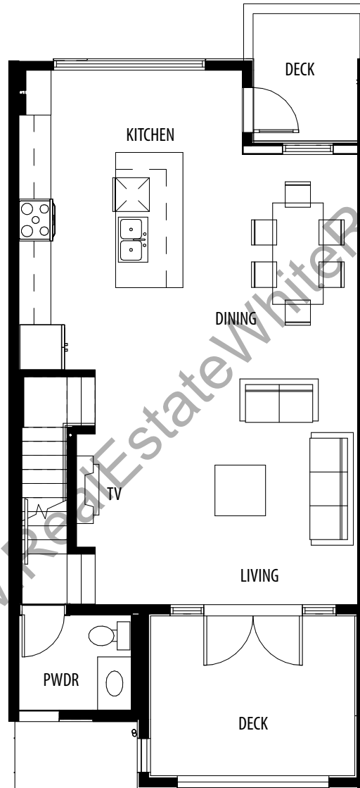
FIRST FLOOR 702 S.F.
