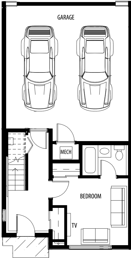
MAIN FLOOR 361 S.F.
