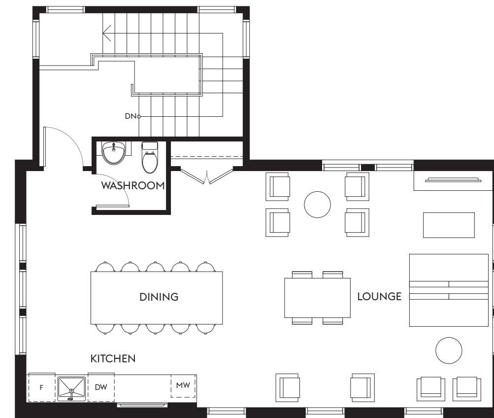
UPPER LEVEL
