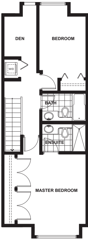
upper level
