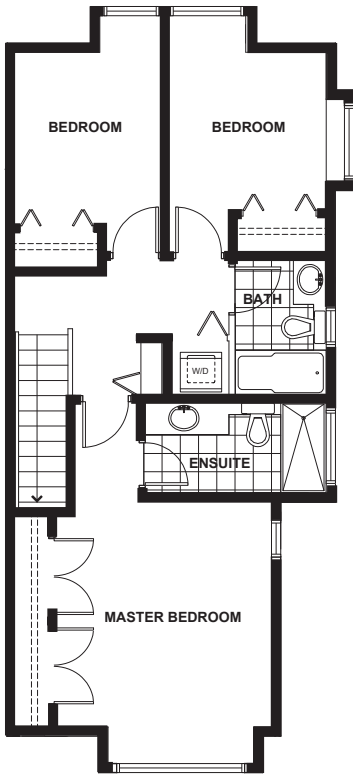
upper level
