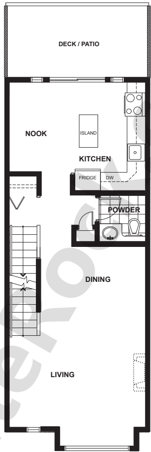
main level
