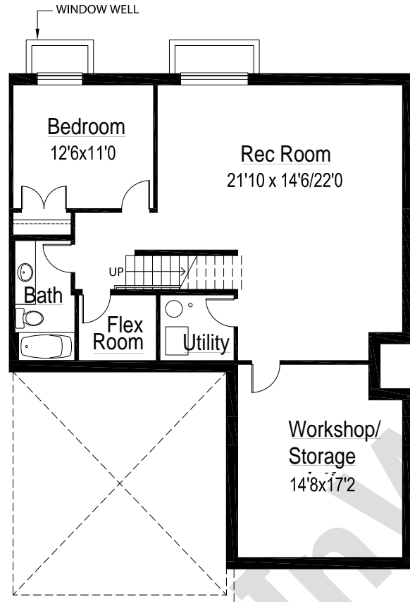
BASEMENT FLOOR: 1,234 sqft. approx.
