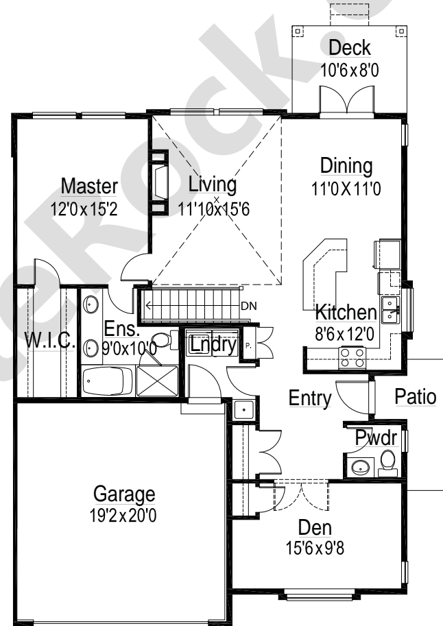
MAIN FLOOR: 1,236 sqft. approx.
