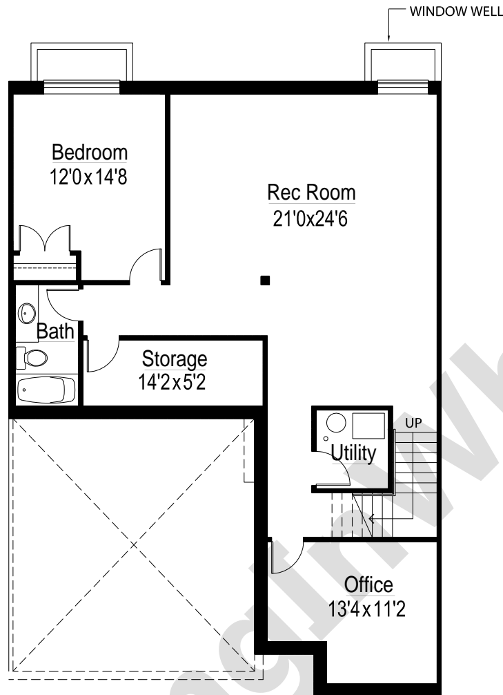
UNFINISHED BASEMENT FLOOR: 1,200 sqft. approx.
