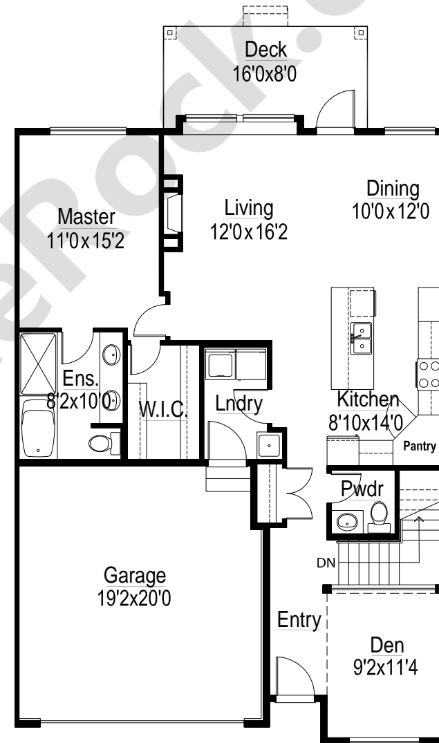
MAIN FLOOR: 1,200 sqft. approx. GARAGE: 400 sqft. approx.
